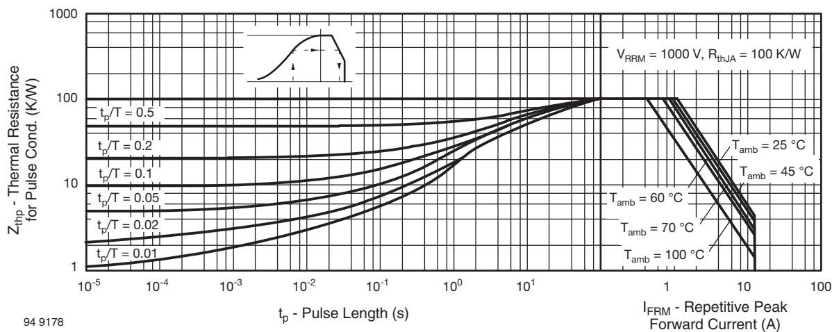
Fig. 7 - Thermal Response
