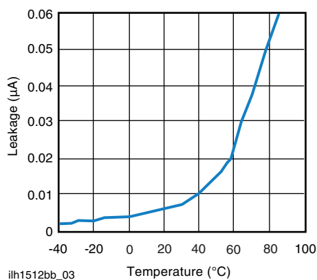
Fig. 4 - Typical Leakage vs. Temperature (Measured across Pin 5 and 6 or 7 and 8)
