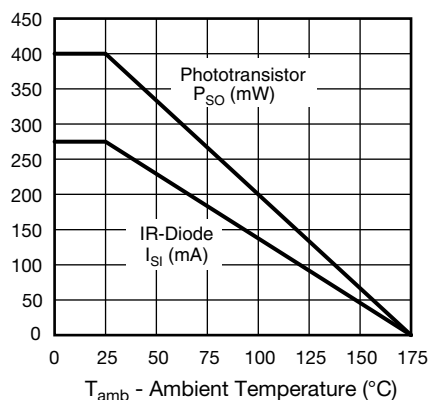
Fig. 1 - Derating Diagram
