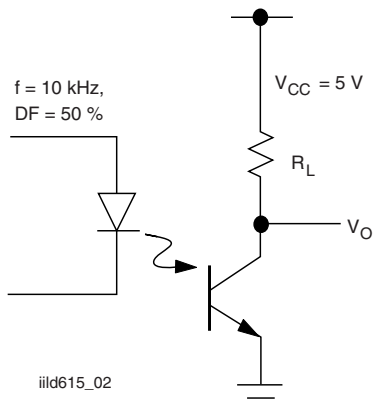
Fig. 3 - Saturated Switching Timing
