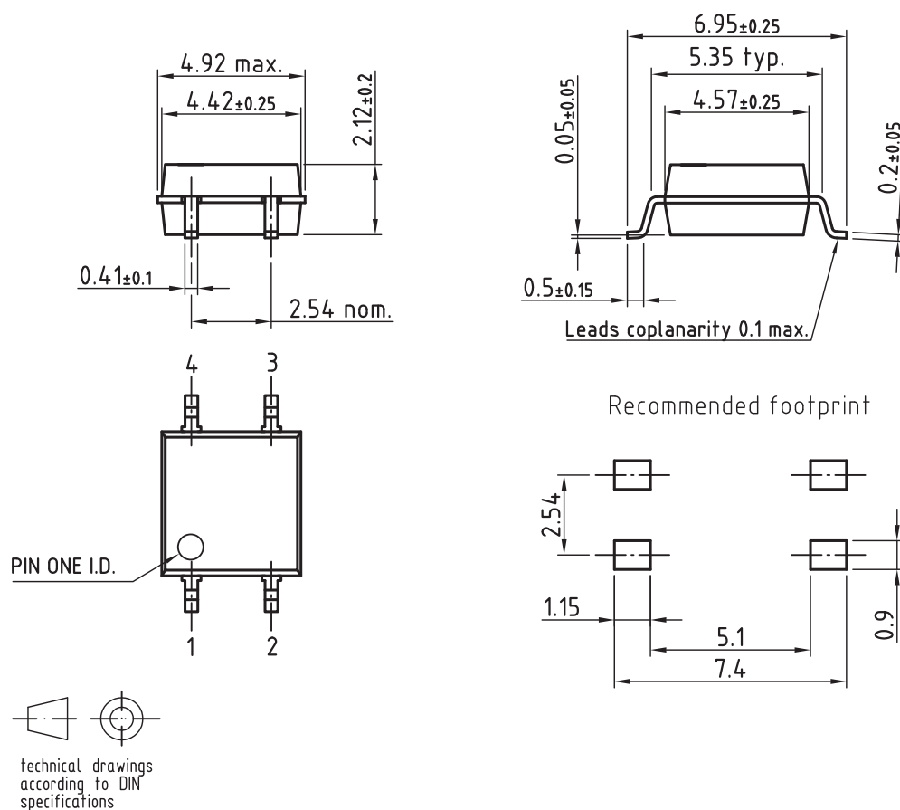
Fig. 14 - Package Drawing
